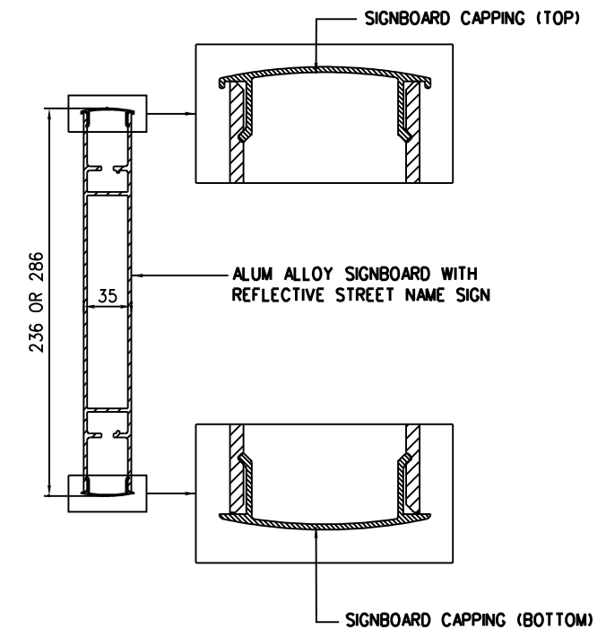
TYPICAL SIGNBOARD WITH CAPPINGS SCALE 1:50
