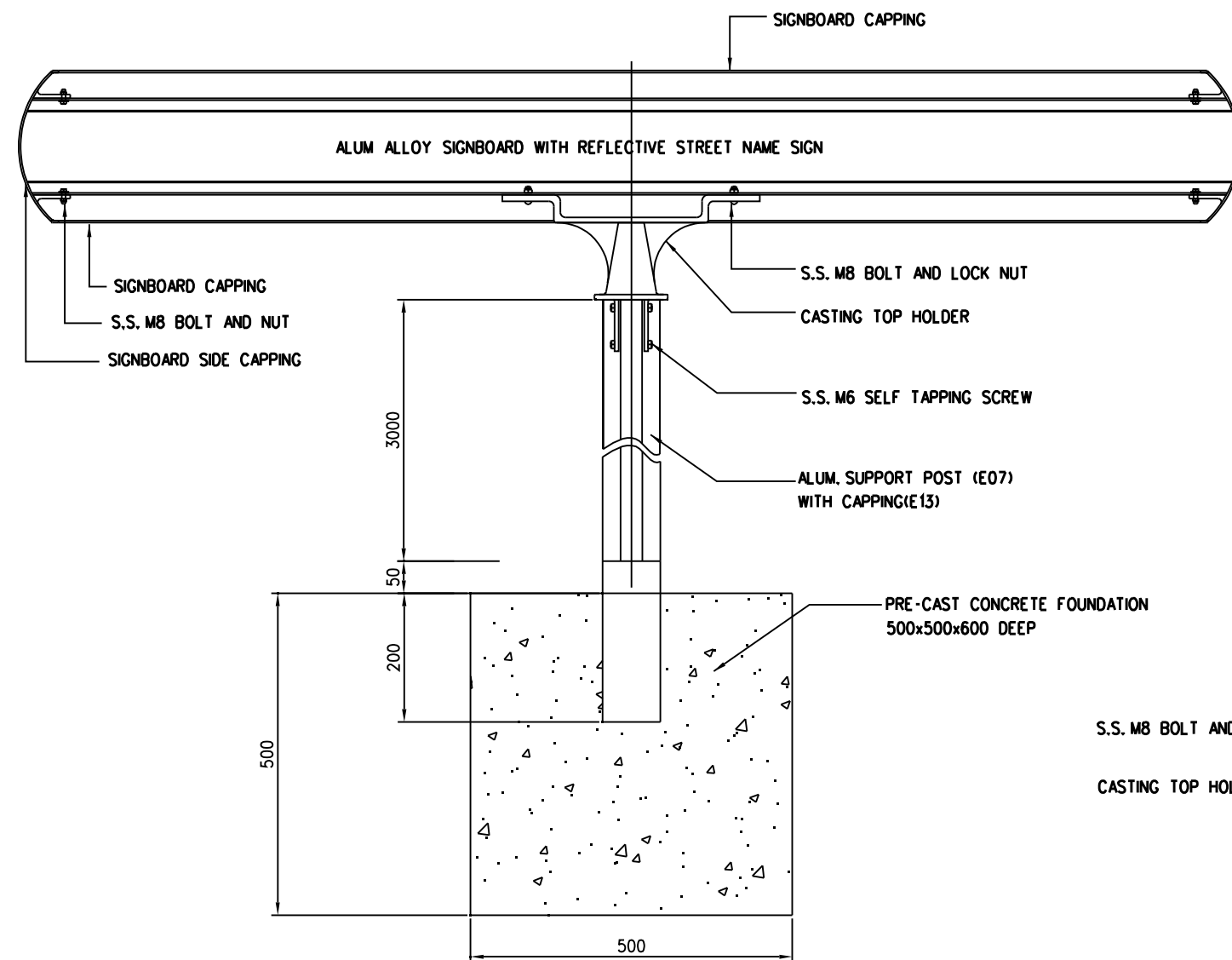
ELEVATION SCALE 1:10
