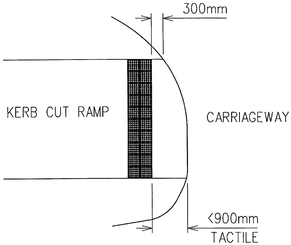
CURVED KERB CUT RAMP - TYPE B
